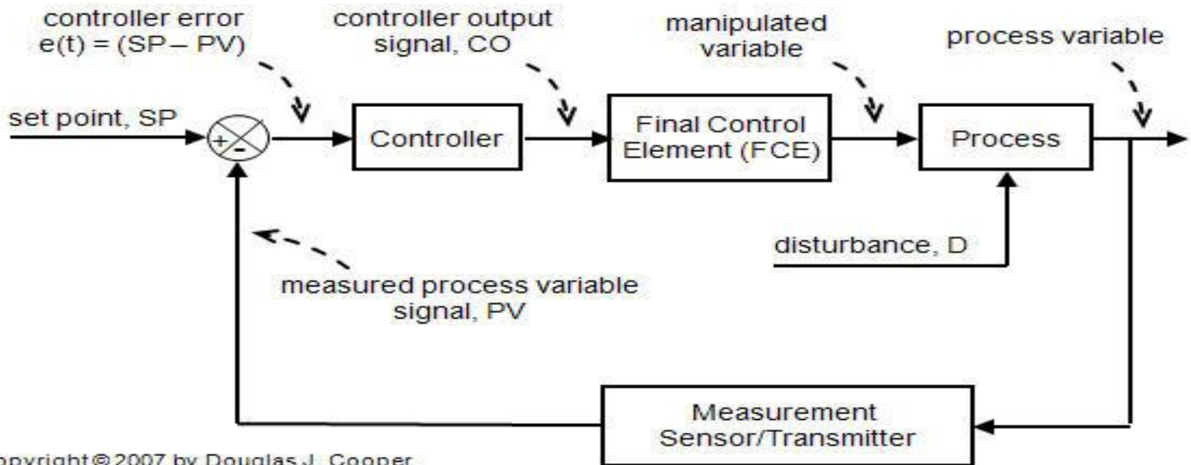
General Control Loop Block Diagram
